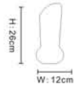
MT1771 / 1T WHITE G9, 1×MAX. 40W
