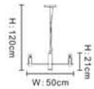
MT1710/6P SATIN NICKEL E14, 6×MAX. 7W(Energy-Saving) G9, 6×MAX. 40W
