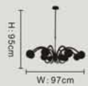
MT1836 / 8+4P SATIN NICKEL G9, 12×MAX. 40W
