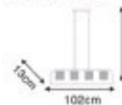
P8061/04A (MC-2) G9 4x40W
